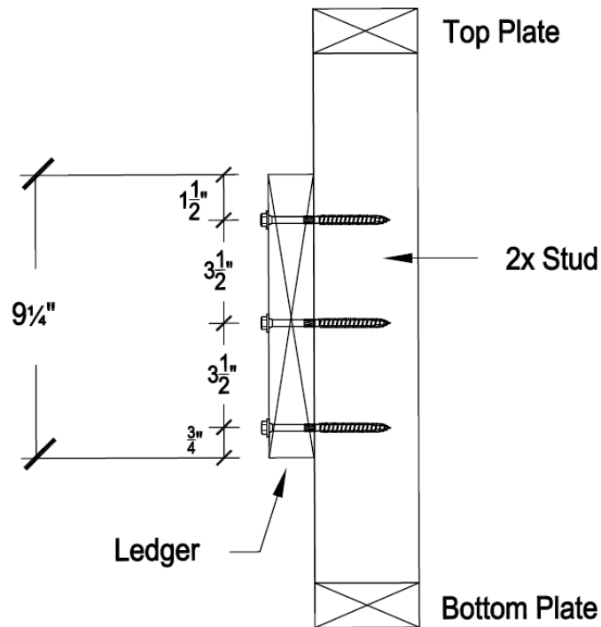
Figure 9. 2 x 10 Ledger with No GWB
