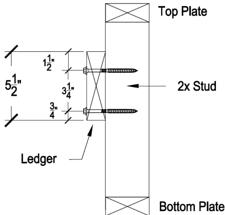
Figure 7. 2 x 6 Ledger with No GWB
