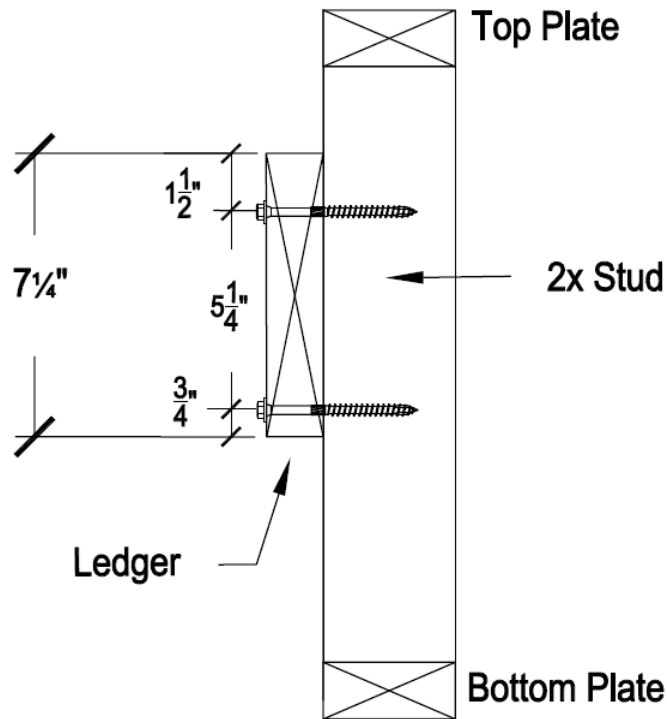
Figure 8. 2 x 8 Ledger with No GWB
