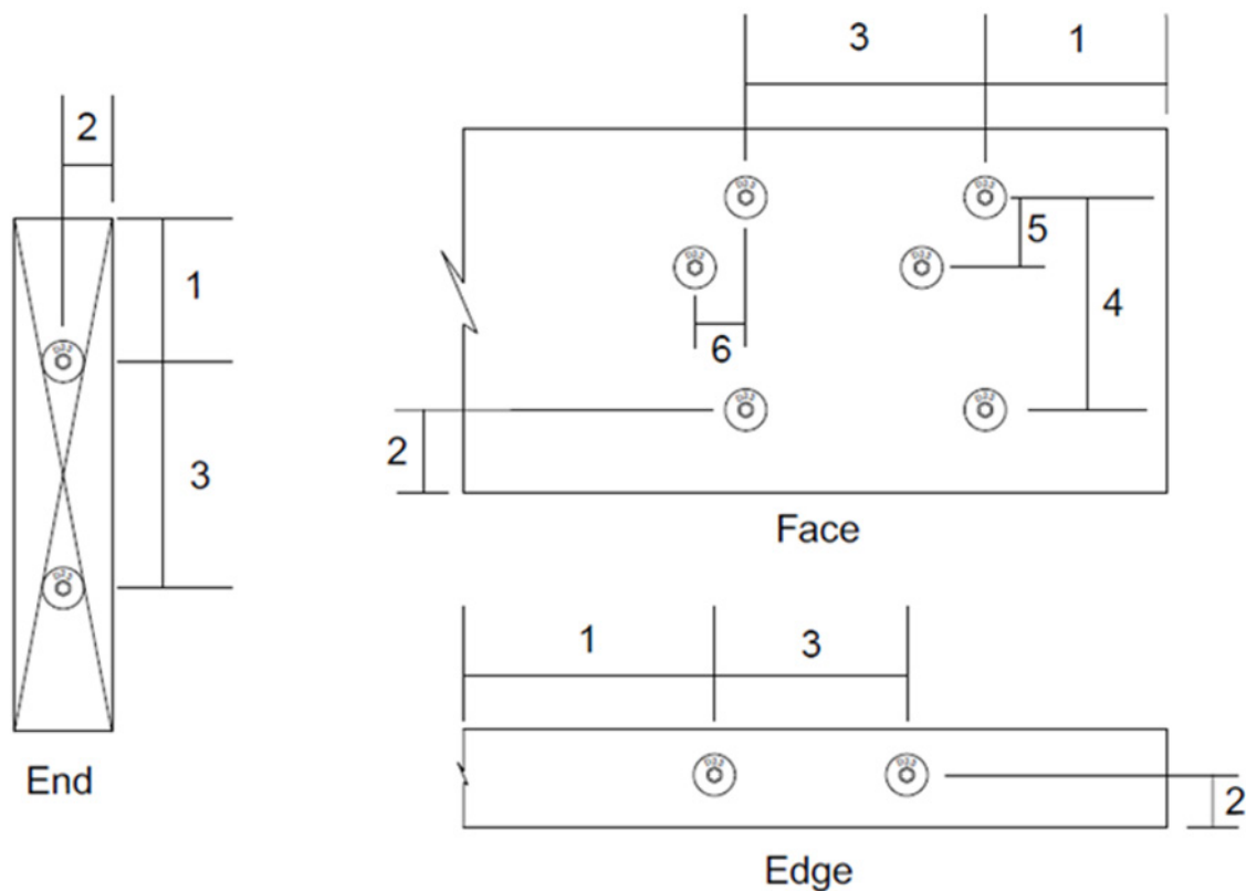
Figure 4. Starborn Structural Screws Spacing Diagram
